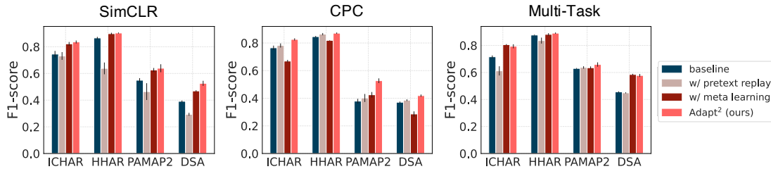
Fig. 6. F1-scores of the ablation study. We compare ADAPT^2 against 1) the baseline self-supervised learning method, 2) the baseline only with pretext replay, and 3) the baseline only with meta-learning. Ten-shot fine-tuning is performed.
