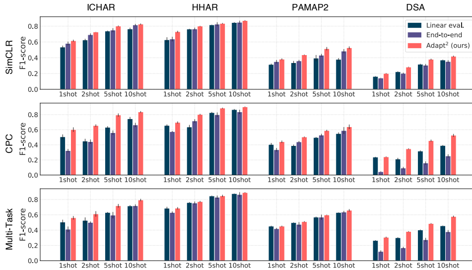
Fig. 5. Average F1-scores of ADAPT^2 , built upon different self-supervised learning methods across different shot numbers (1, 2, 5, 10).
