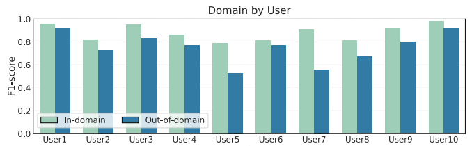
Fig. 1. Efficacy of CPC [9] pre-trained models on ICHAR [18] dataset, comparing F1-scores between in-domain and out-of-domain pre-training scenarios. Ten participants with different devices are shown as domains. Domain shifts deteriorate the performance of self-supervised models in heterogeneous environments.
