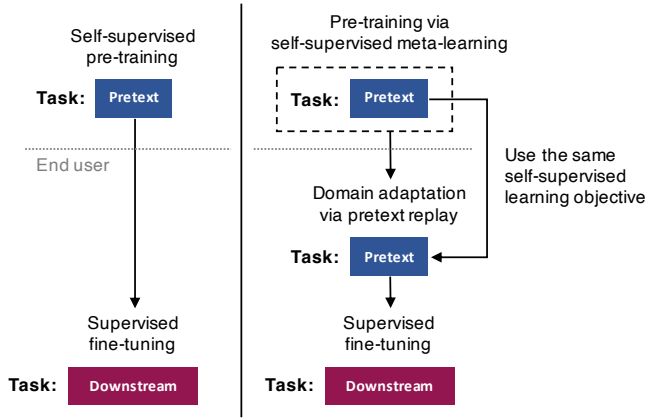
Fig. 2. A high-level comparison between the standard self-supervised learning (left) and ADAPT^2 (right).
