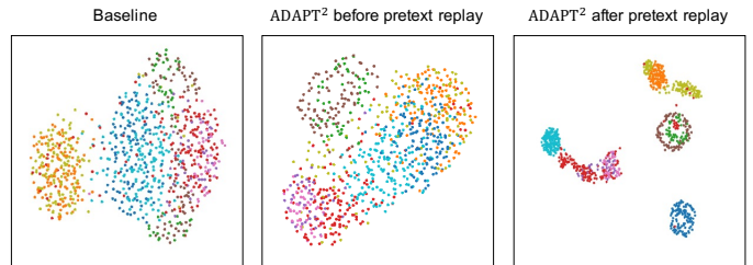
Fig. 7. 2D UMAP visualizations of embeddings from CPC pre-trained models. Embeddings are color-coded by class.
