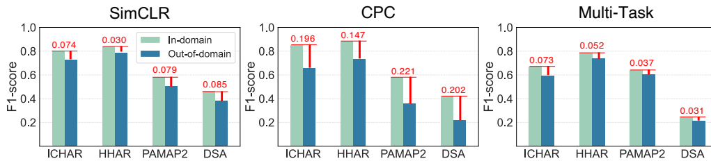
Fig. 8. Fine-tuning performance comparison between models pre-trained in-domain and out-of-domain settings. Ten-shot fine-tuning is performed for all settings. Performance drops between the settings are shown in red.
