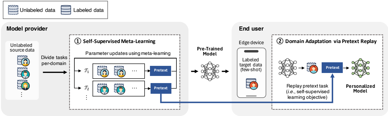
Fig. 3. Overview of ADAPT^2 framework.
