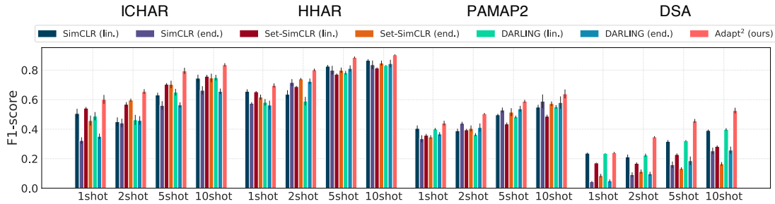
Fig. 4. Average F1-scores of ADAPT^2 and the baselines across different shot numbers (1, 2, 5, 10).
